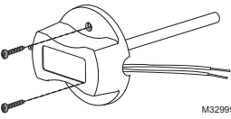
Fig. 6. Mounting Discharge/Return Air Sensor.
