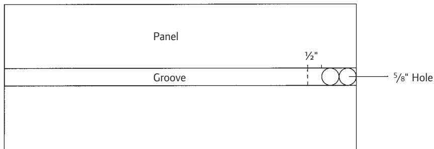
Figure 19: Drill Two Holes to Create a Rectangular Slot in the Subfloor
