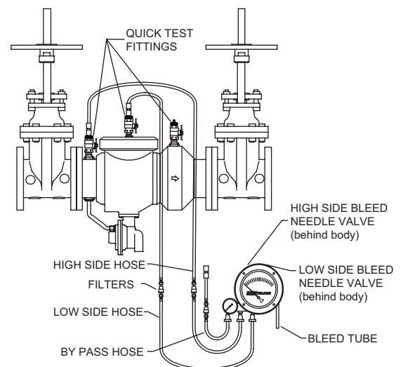
MODEL 4" 375 SHOWN
