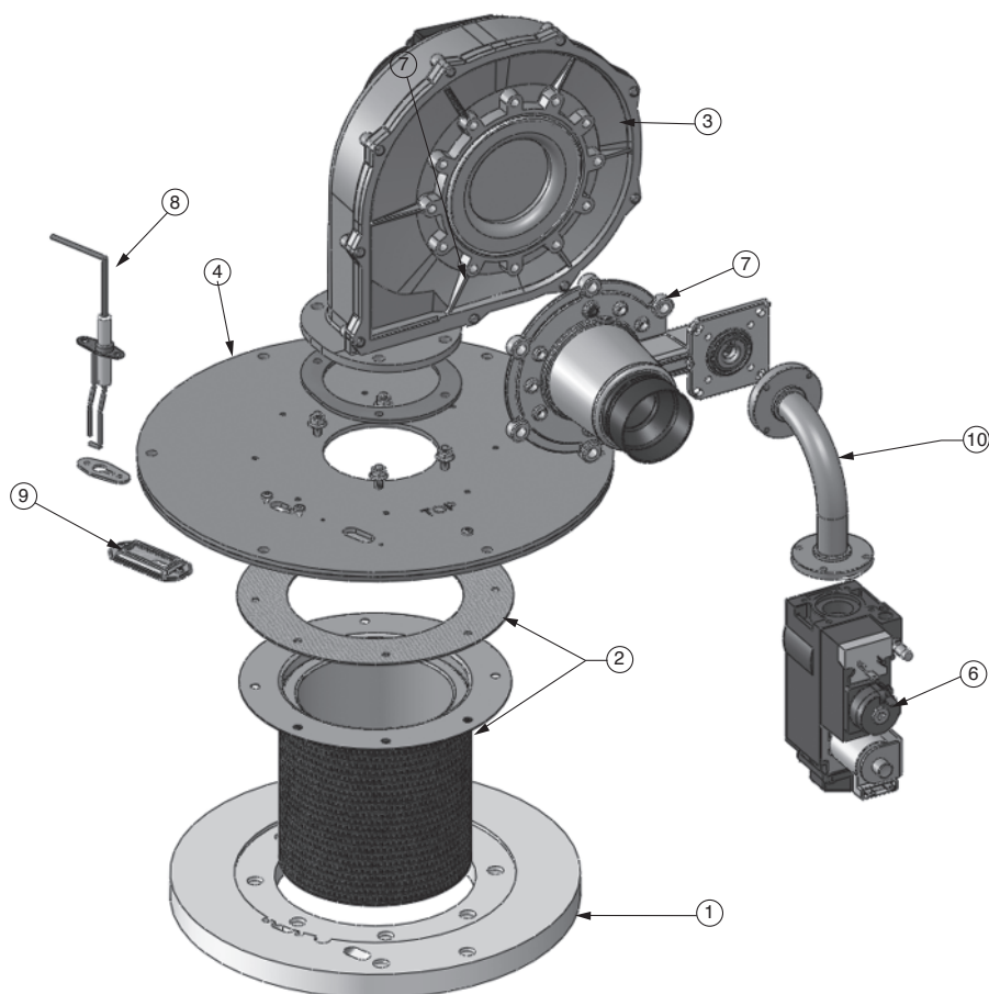
Fig. 40: PRESTIGE Solo 399 Burner Components
