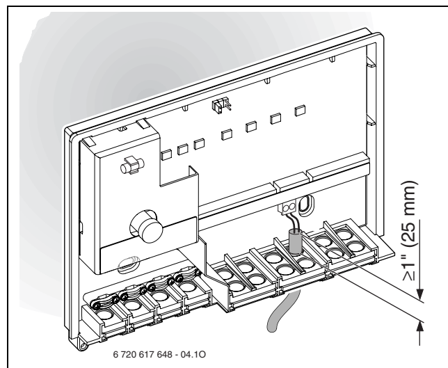
Fig. 9 Splash-proof
