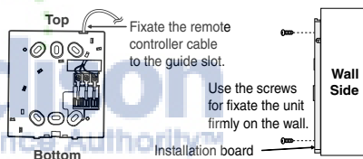
<Front side of installation board>
