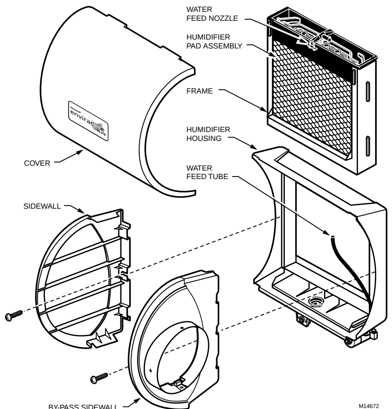
Fig. 2. Humidifier components.
