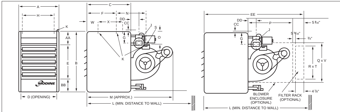
Figure 20.1 - Dimensional Drawings
