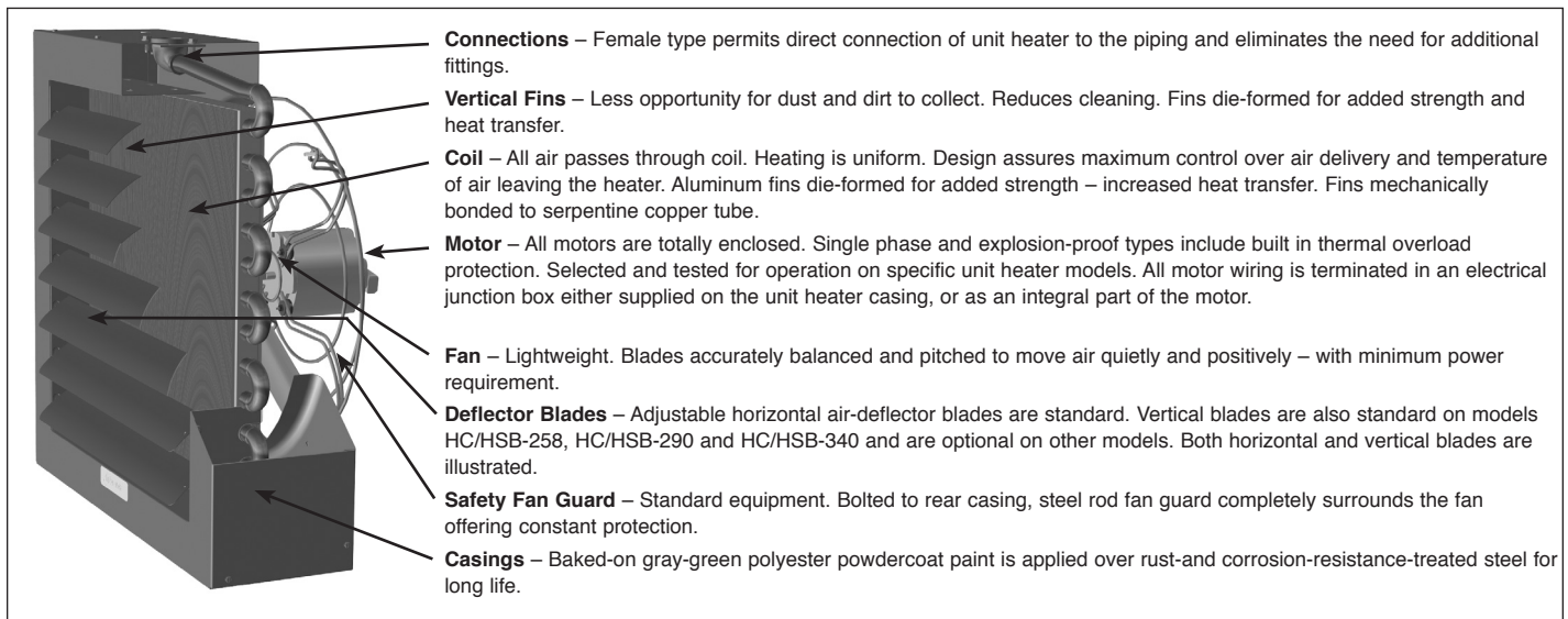
Figure 4.1 - Unit Features
