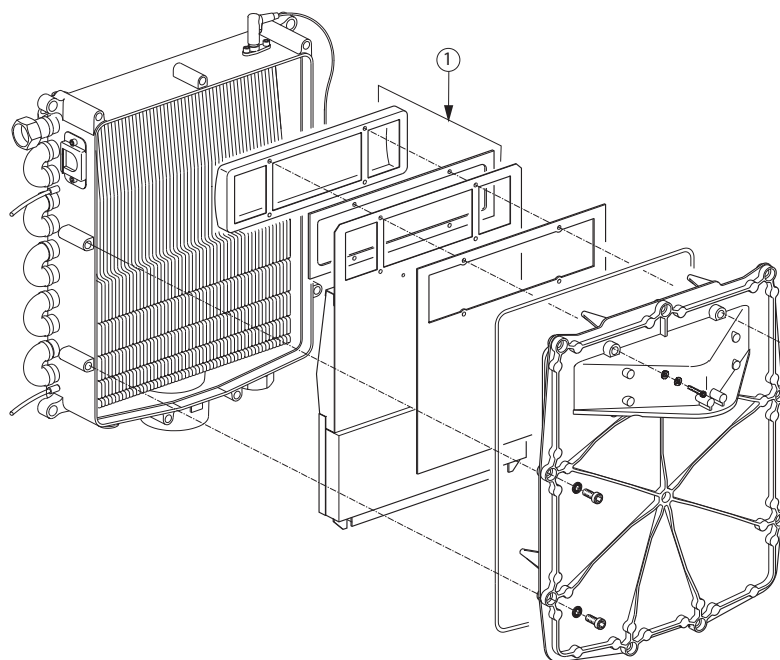
Fig. 32 : CHALLENGER Burner Components
