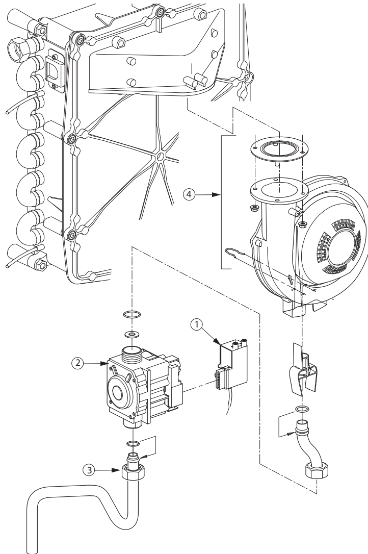
Fig. 31 : CHALLENGER Blower & Gas Valve Components
