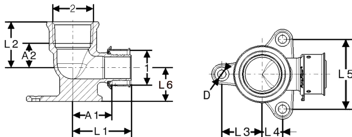
Viega PEX Press Drop Ear Elbows
