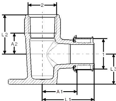
Viega PEX Press Fire Sprinkler Elbow (Double)
