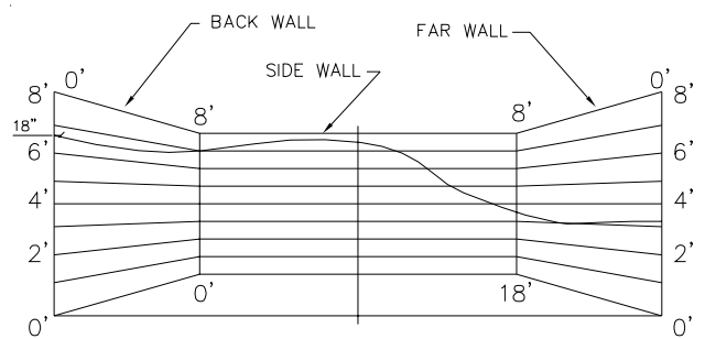
14.6 P.S.I. - 31 G.P.M. 16' x 18' (HALF PATTERN)
