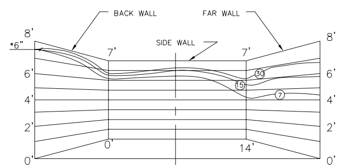
17/32" Orifice - K = 8.1
