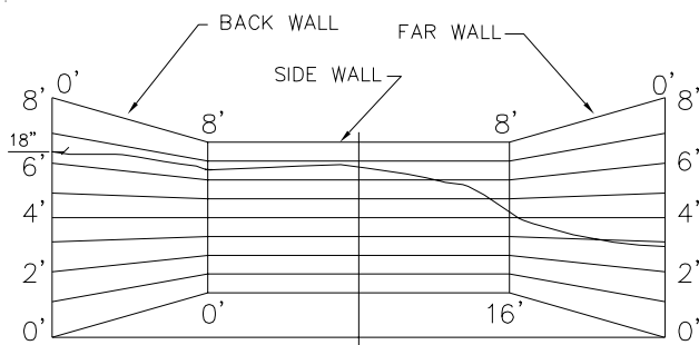
11.9 P.S.I. - 28 G.P.M. 16' x 16' (HALF PATTERN)
