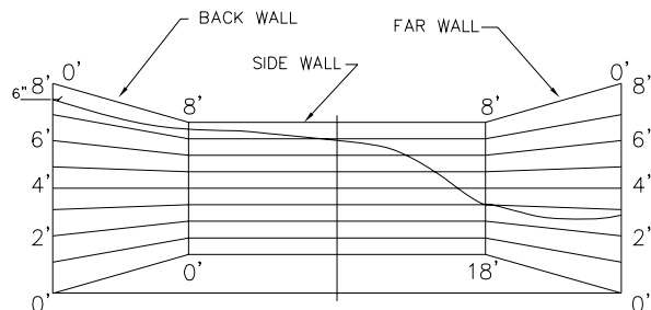
26.8 P.S.I. - 29 G.P.M. 16'x18' (HALF PATTERN)
