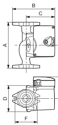
UPS 26-99 BFC
