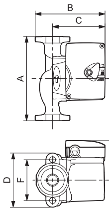
UPS 26-99 FC
