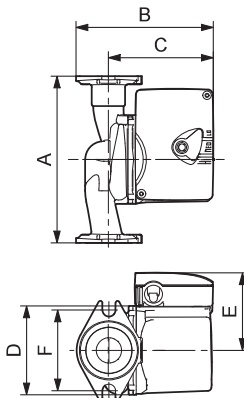
UPS 15-35 SFC
