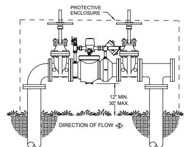
OUTDOOR INSTALLATION
