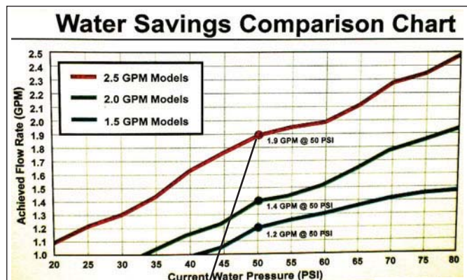
Average Flow Rate for 2.5 GPM Max- rated head is 1.9 GPM
