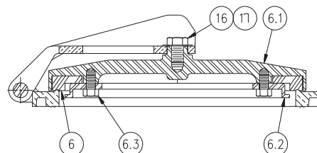
10" Disc Assembly (250mm)
