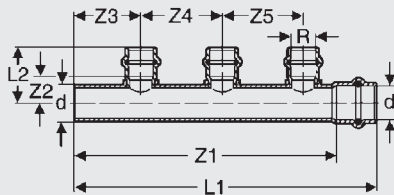
Bronze PEX Press ProPress Copper Manifolds
