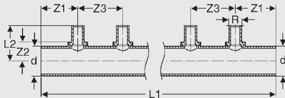
PEX Press Braided Copper Manifold - Headers
