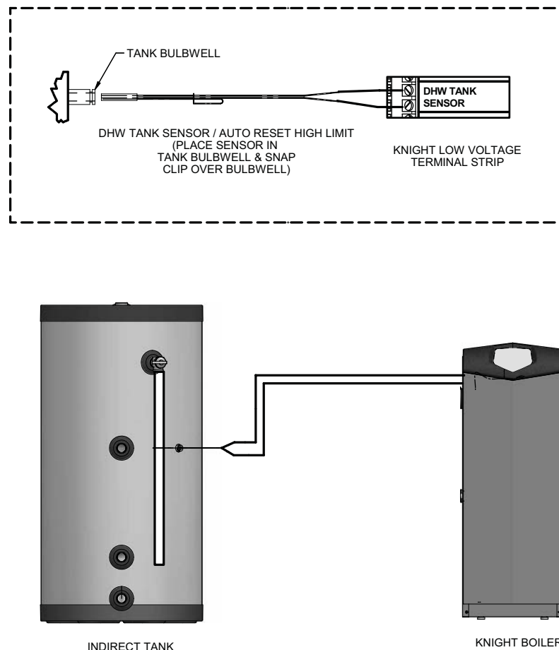
Figure 5-1 Indirect Water Heater Controlled Using Tank Sensor
