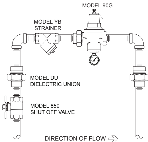
TYPICAL INSTALLATION
