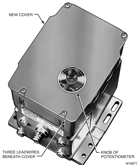
Fig. 1. Q209E Modutrol IV Manual Potentiometer (cover-mounted).
