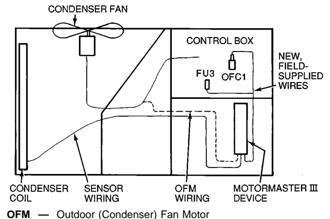
Fig. 6 — Wire Routing (208/230-V Shown)
