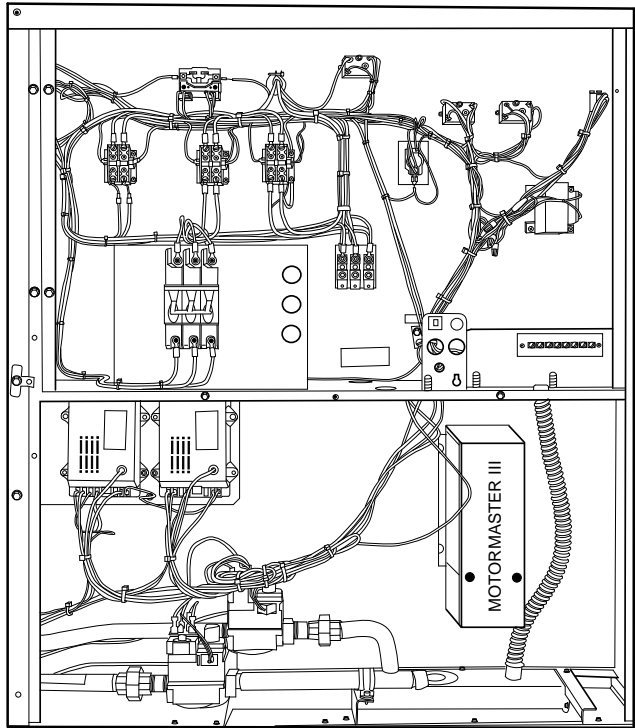
Fig. 3 — Motormaster III Controller Installed (48TJE028 Shown)
