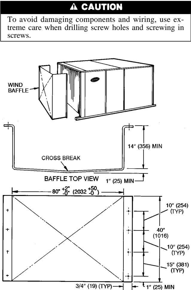
Fig. 2 — Wind Baffle Details
