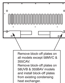
Fig. 4 - Block-off Plates
