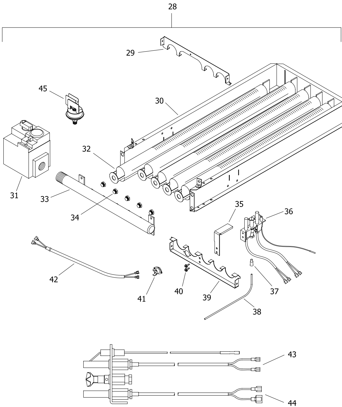
THERMOPILE DETAIL
