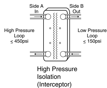
Diagram 3-High Pressure Isolation
