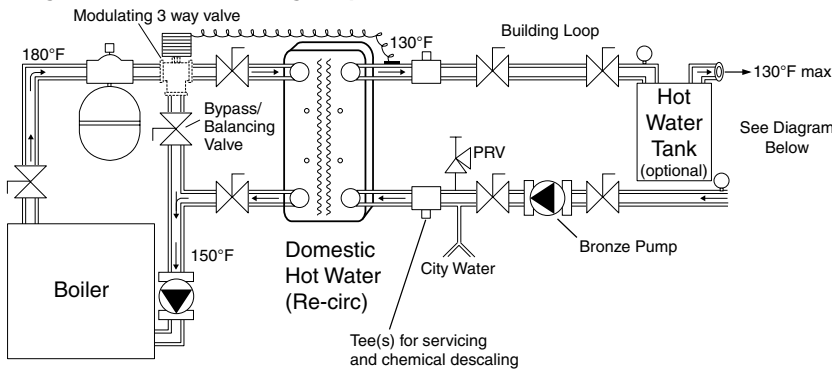
Diagram 2-Recirc to Building Loop
