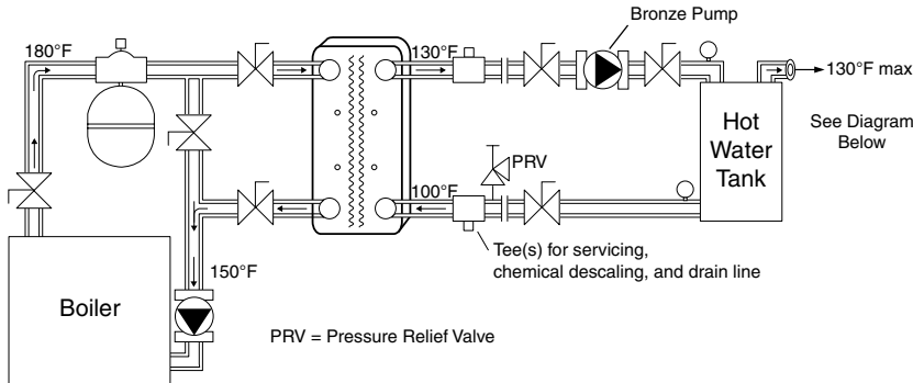
Diagram 1-Recirc to Tank
