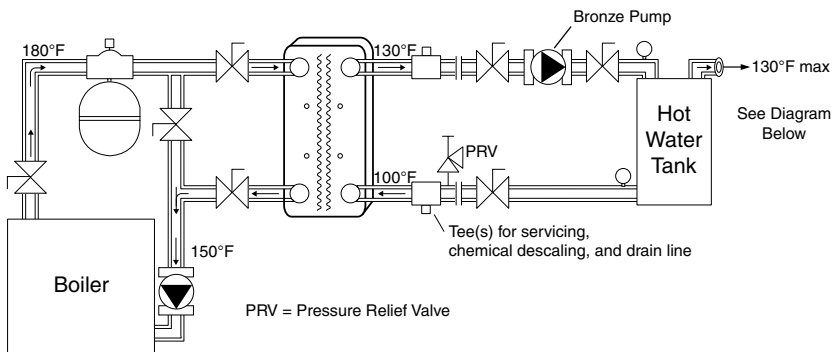
Diagram 1-Recirc to Tank
