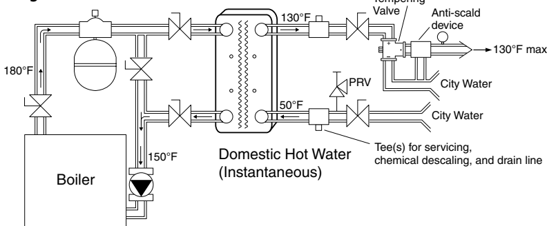
Diagram 3-Instantaneous
