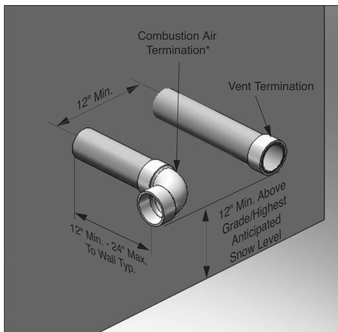
Fig. 13: Direct Vent - Sidewall Termination of Vent and Combustion Air Piping with Coupling Vent Termination
