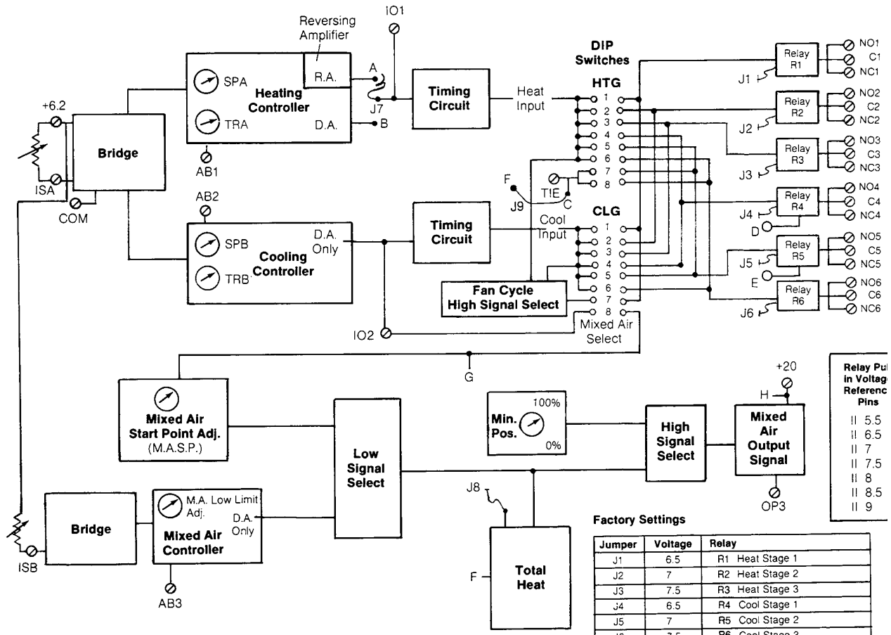
Controller Block Diagram
