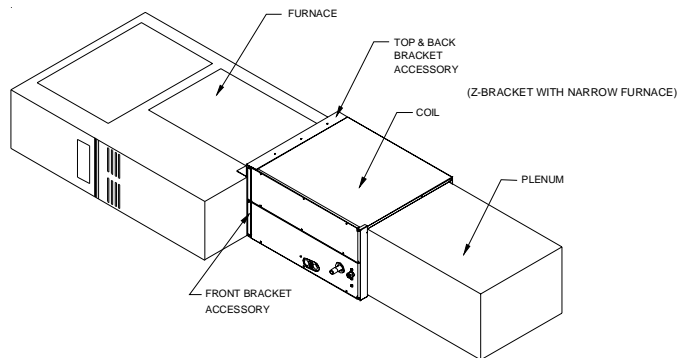
Figure 3 Installation of Furnace, Coil and Plenum
