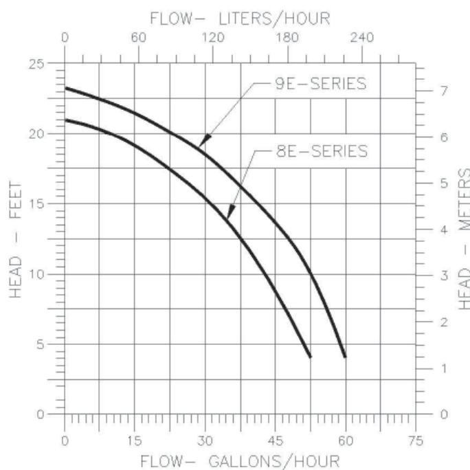
Figure 3 - Performance Curve/Courbe de Performances/ Curva de Rendimiento
